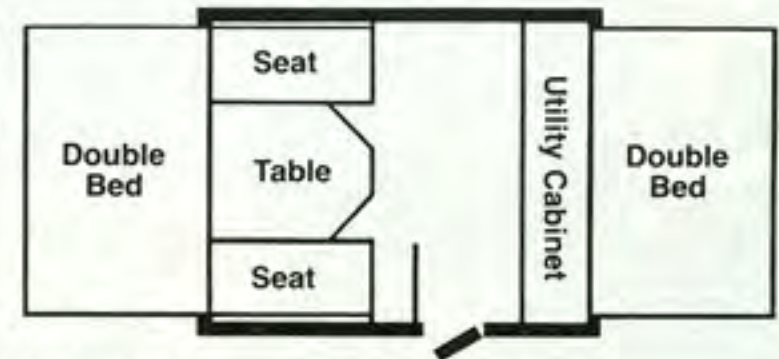
Starlite 6 Dimensions/Weights
