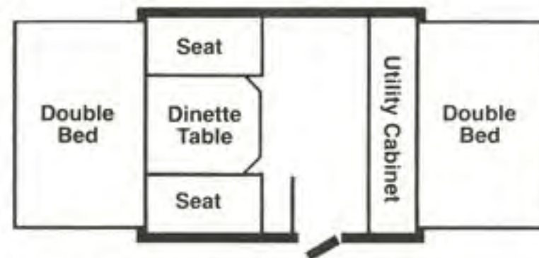
Starlite 6 Dimensions/Weights
